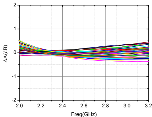
Amplitude Variation
