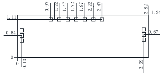
Assembly Diagram
