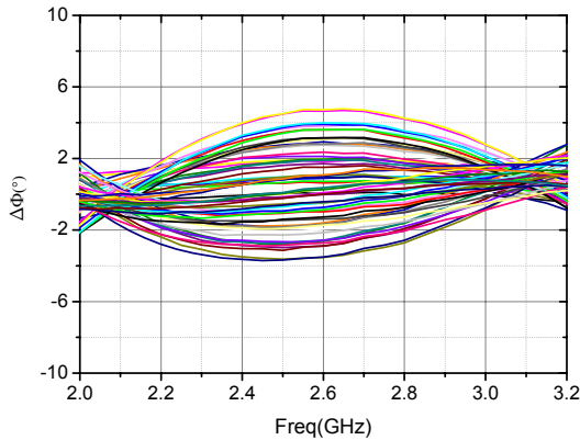
Phase Error
